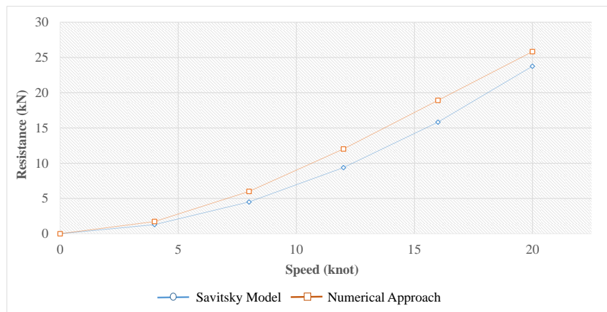
Fig. 11. Savitsky's mathematical model for the monohull with low fin the ratio of 30 deg (Model 2).
