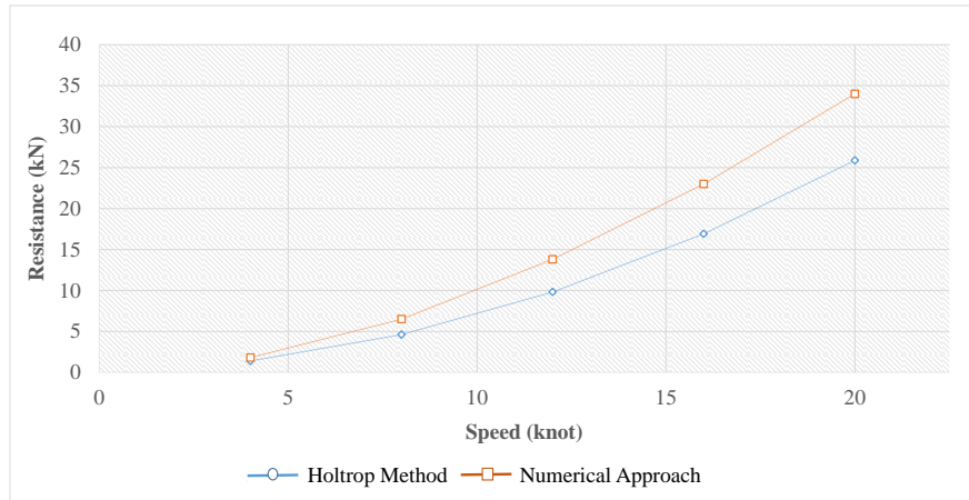
Fig. 15. Results of the Holtrop method for the monohull with daggerboard fin of 30 deg (Model 3).
