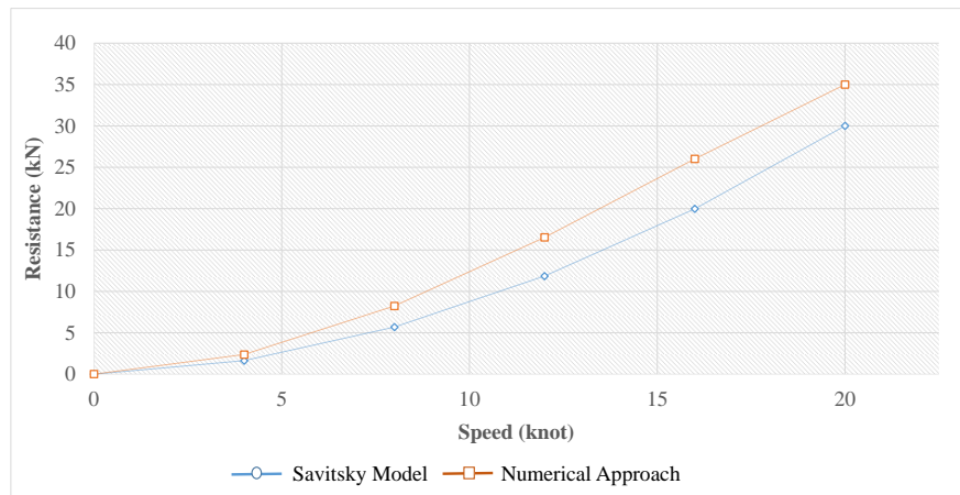
Fig. 12. Savitsky's mathematical model for the monohull with daggerboard fin of 30 deg (Model 3).
