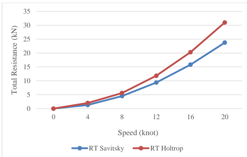
Fig. 17. Savitsky model vs. Holtrop method: the monohull with low fin the ratio of 30 deg (Model 2).
