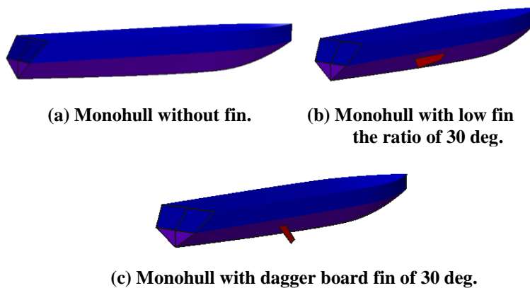
Fig. 9. Hull variation of the new fishing vessel design.
