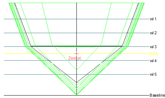
Fig. 6. Body plan of the new vessel design.
