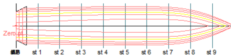
Fig. 7. Breadth plan of the new vessel design.
