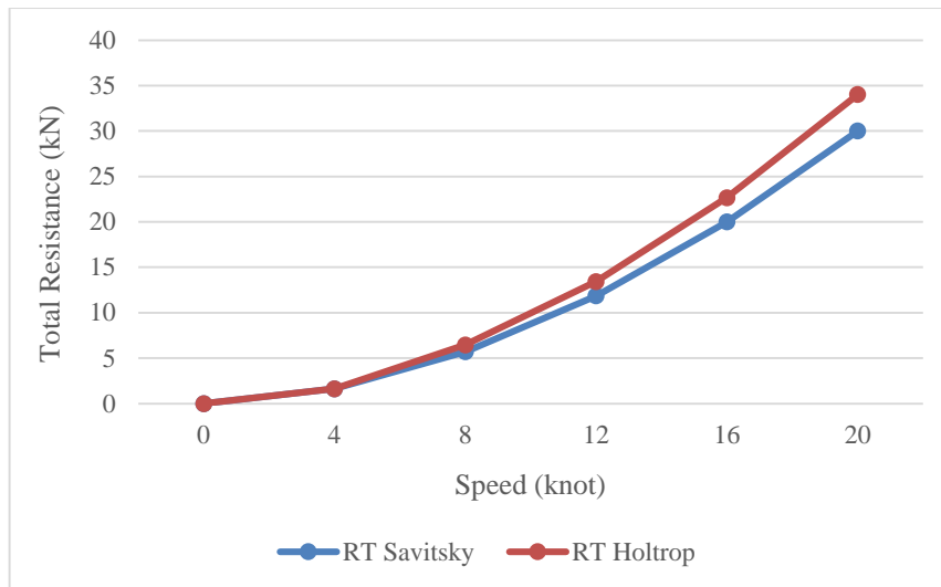
Fig. 18. Savitsky model vs. Holtrop method: the monohull with daggerboard fin of 30 deg (Model 3).
