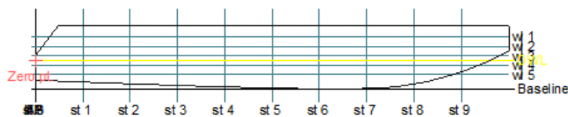
Fig. 8. Sheer plan of the new vessel design.
