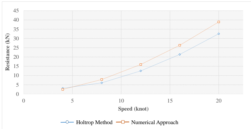
Fig. 13. Results of the Holtrop method for the Monohull without fin (Model 1).
