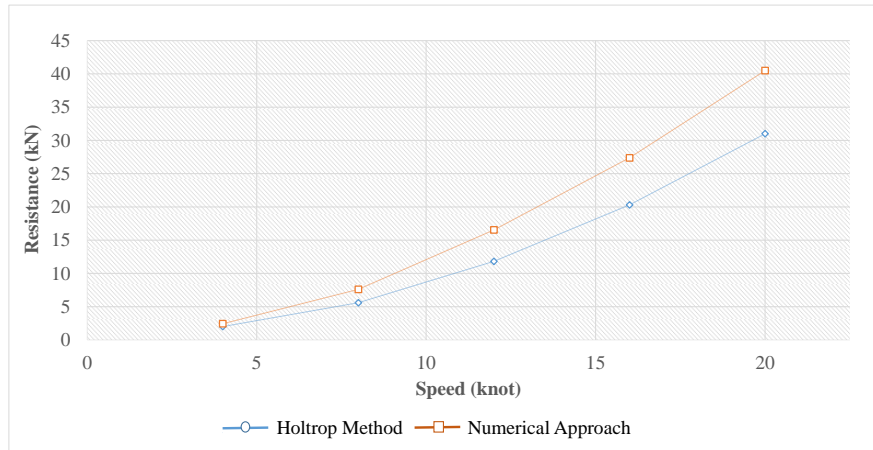
Fig. 14. Results of the Holtrop method the monohull with low fin the ratio of 30 deg (Model 2).
