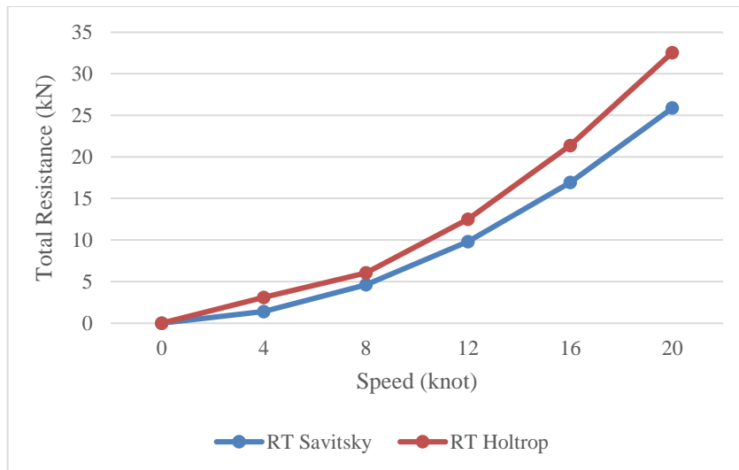
Fig. 16. Savitsky model vs. Holtrop method: the monohull without fin (Model 1).
