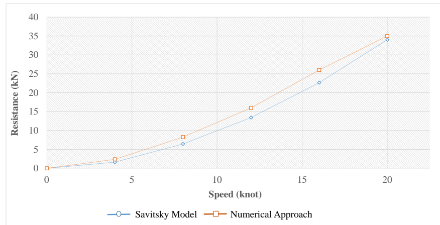
Fig. 10. Savitsky's mathematical model for the monohull without fin (Model 1).
